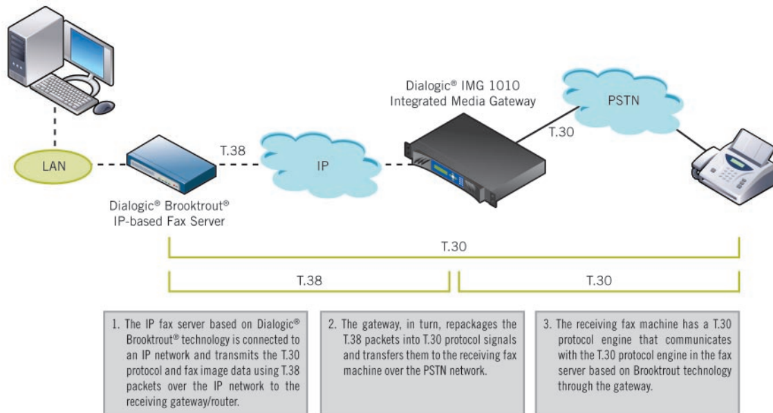
Figure 2. Using Dialogic® Brooktrout® IP-Enabled Fax Server Eliminates the Second Gateway
